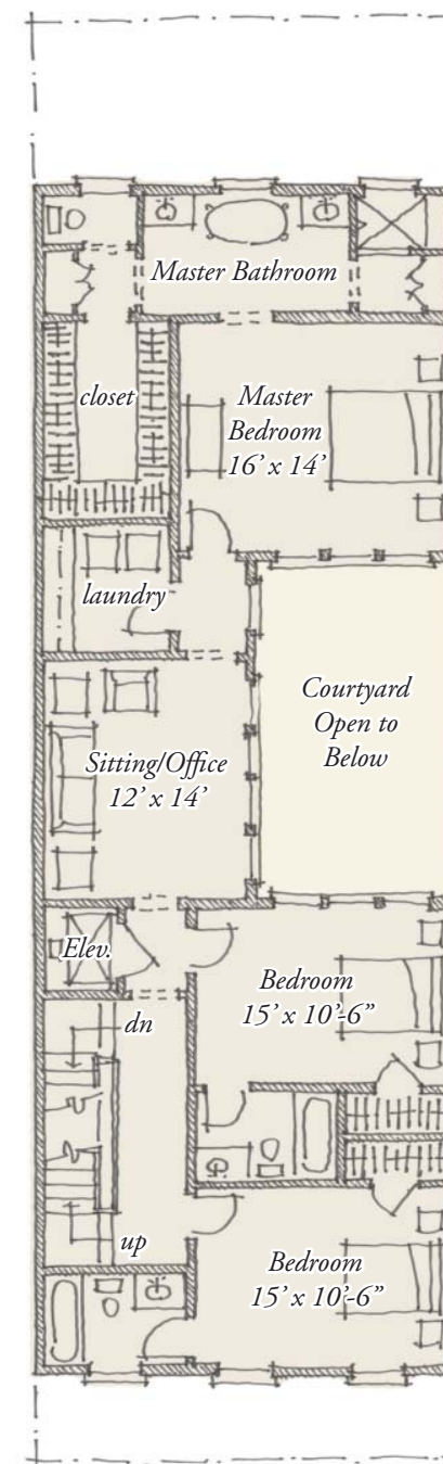
Upper Floor Option A 1,510 S.F.
